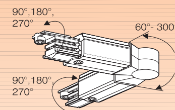
XTS 36
