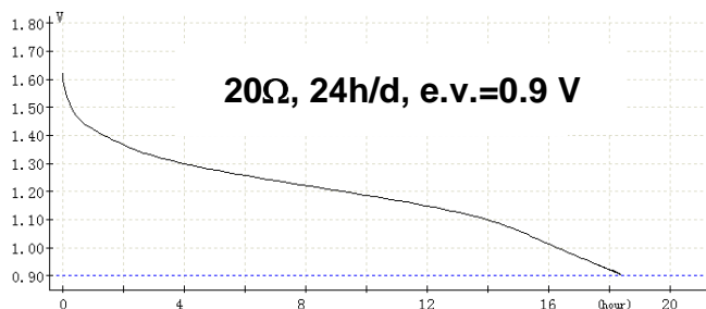
Chart 1. Discharge diagram
